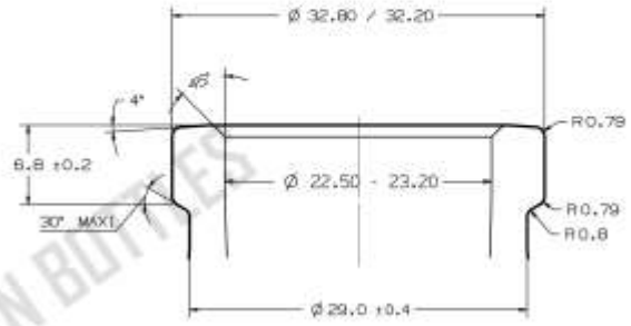
Neck Finish Detail
